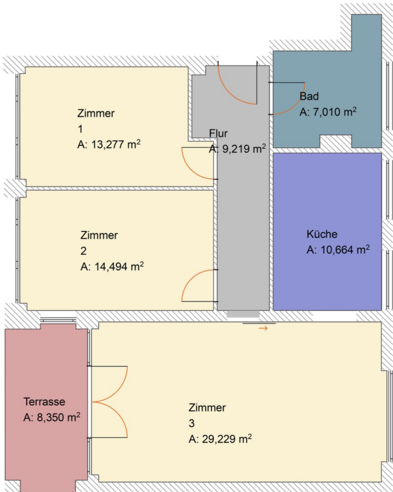
Floor Plan
